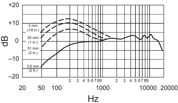
Frequency Response
