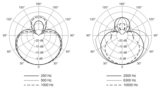
Polar Pattern
